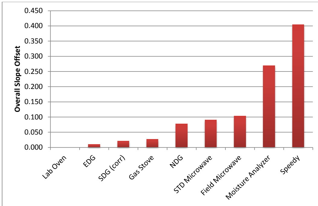
Figure 21. Average slope offset to laboratory oven correlation for each tested device.
