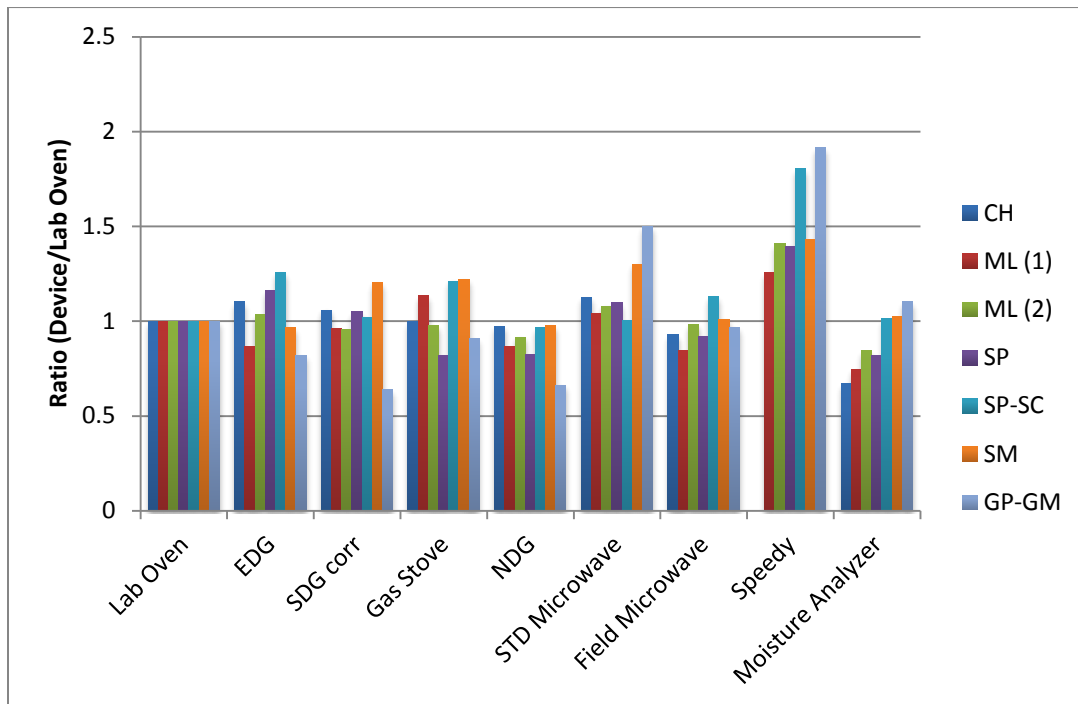
Figure 22. Ratio of average device to laboratory oven moisture content for each soil tested.
